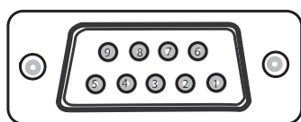
RS-232C port of the computer
